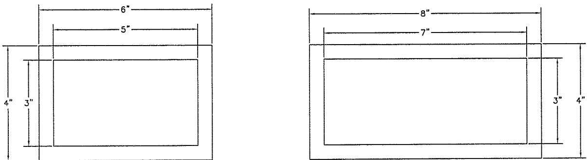
TEFLON PLATE DETAIL
