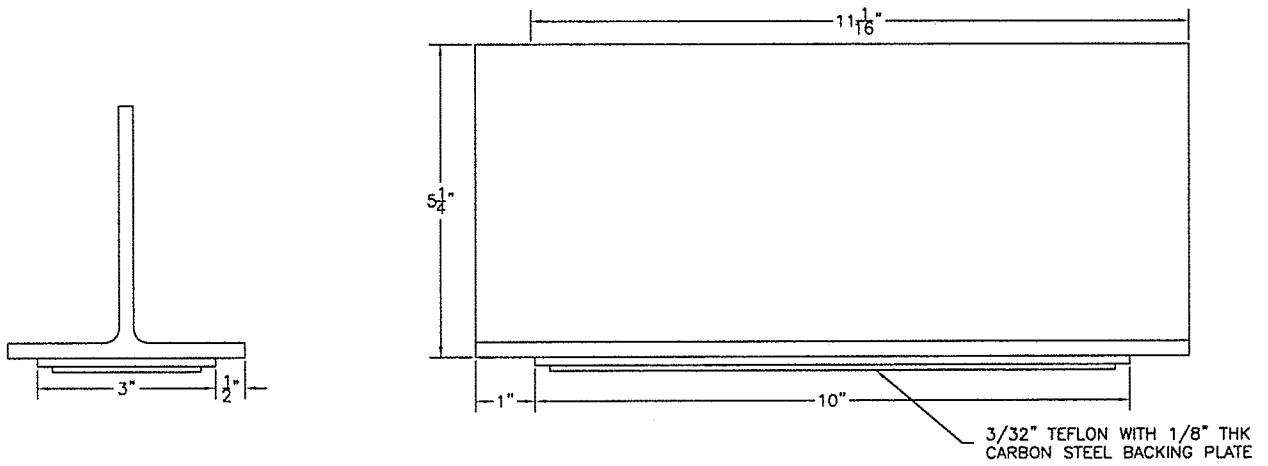
TEE DETAIL
