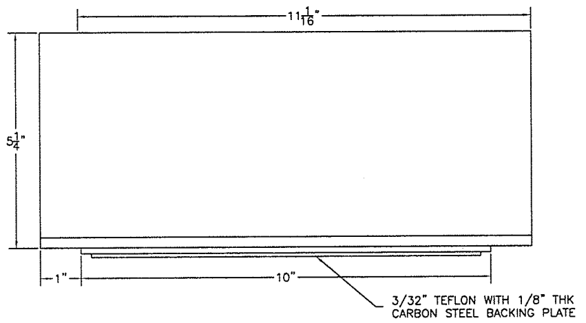
TEE DETAIL
